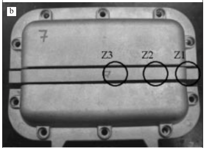
Fig. 10 – Definition of the regions to be investigated in the safety box (a) and cover (b).
