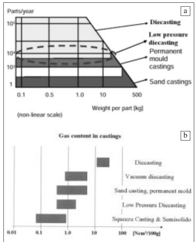
Fig. 1 – Field of convenience of foundry processes as a function of production rate and casting weight (a); comparison of foundry processes in terms of gas content in castings (b).
